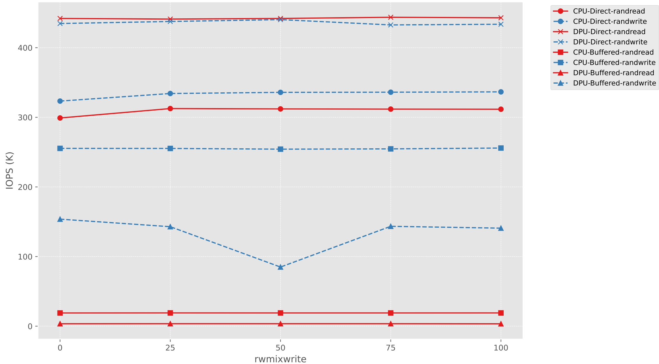
IOPS vs rwmixwrite (CPU vs DPU, Direct vs Buffered)
